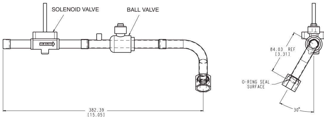
TUBE ASSEMBLY 00PSN500171700AA
